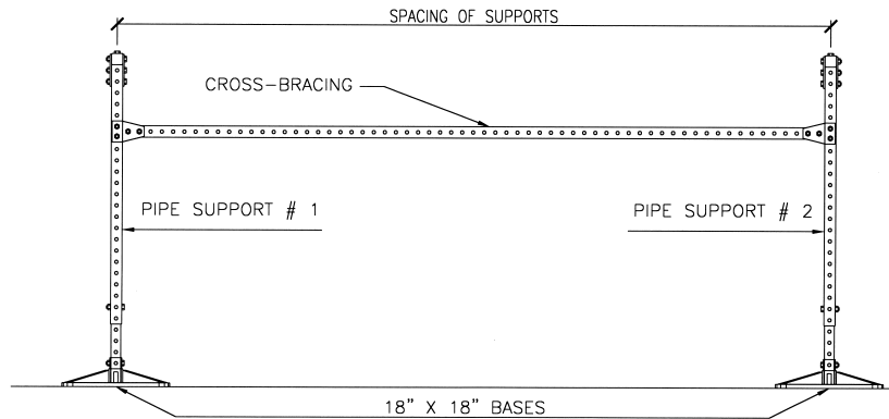
Straight Bracing for pipes 24" above the roof surface and higher.
