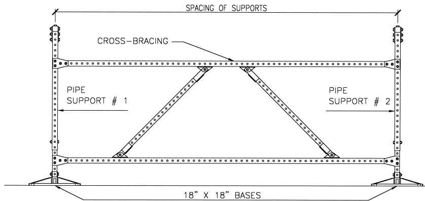
"K" bracing for pipes 24" above the roof surface and higher.
